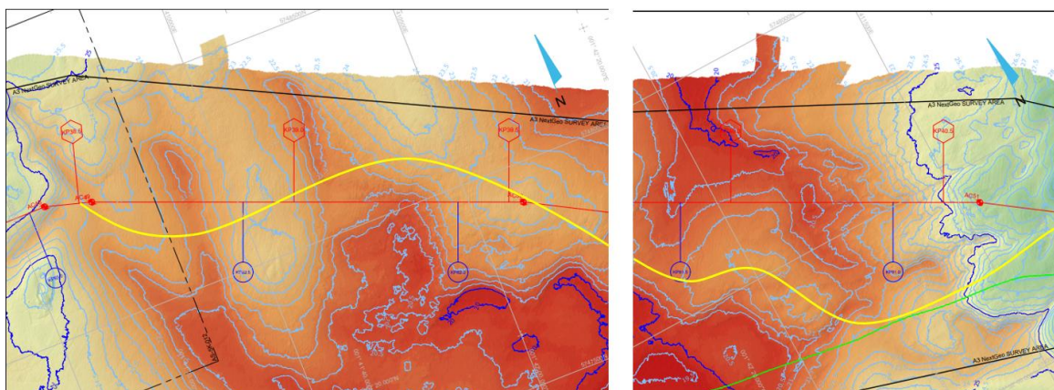
Plate 4.2 Example of micro-routing to link the deepest area of the route corridor (yellow), as opposed to the surveyed Route Position Line (RPL) shown in red with the Kilometre Posts.
